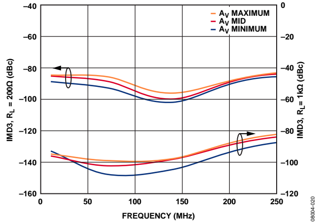
Figure 12. Two-Tone Output IMD vs. Frequency, Output Level at 2 V p-p Composite, R_L = 200 \Omega and R_L = 1 \text{ k}\Omega
