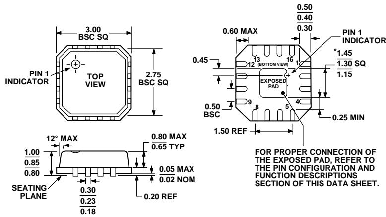
Figure 48. 16-Lead Lead Frame Chip Scale Package [LFCSQ_VQ] 3 mm x 3 mm Body, Very Thin Quad (CP-16-2) Dimensions shown in millimeters
