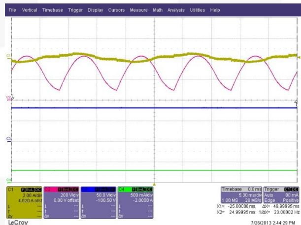
Figure 40. V IN = 300 V AC / 50 Hz, 50% Dim
